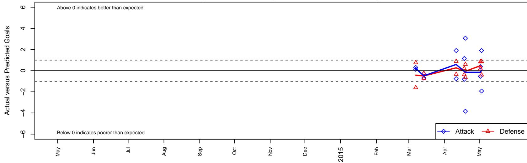
PVSC Crew B97 Dots are actual minus expected GF (blue circles) and GA (red triangles). Blue line is smoothed change in attack strength. Red is smoothed change in defense strength.
